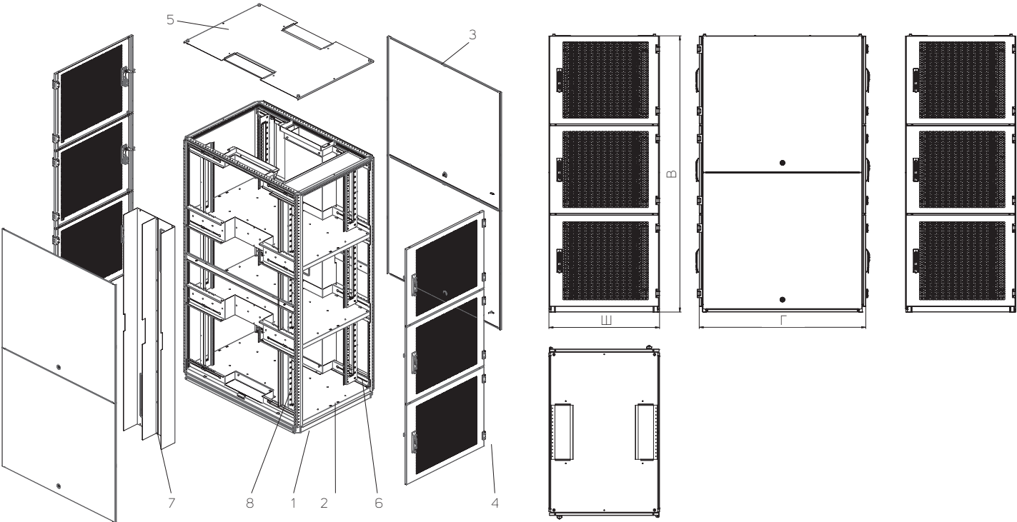
RB1-42-80/120-3
